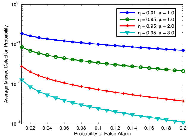
Fig. 2. \bar{P}_m vs P_f ROC curve for for different values of \eta and \mu with u = 4 and \bar{\gamma} = 15 dB.
