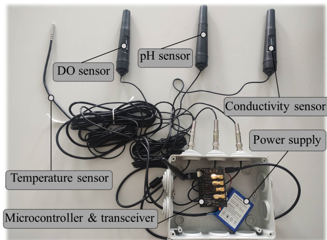
Fig. 3. Wireless Sensor Node
