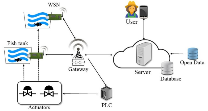
Fig. 1. System Layout
