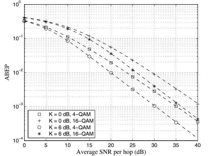
Fig. 4. ABEP of 4 and 16-QAM in Rician/Rayleigh fading. Dashed lines and “markers” denote theoretical and simulated ABEPs respectively.
