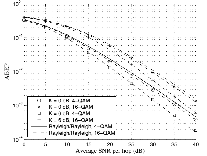
Fig. 3. ABEP of 4 and 16-QAM in Rayleigh/Rician fading. Dashed lines and “markers” denote theoretical and simulated ABEPs respectively.
